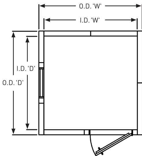
Typical Plan
